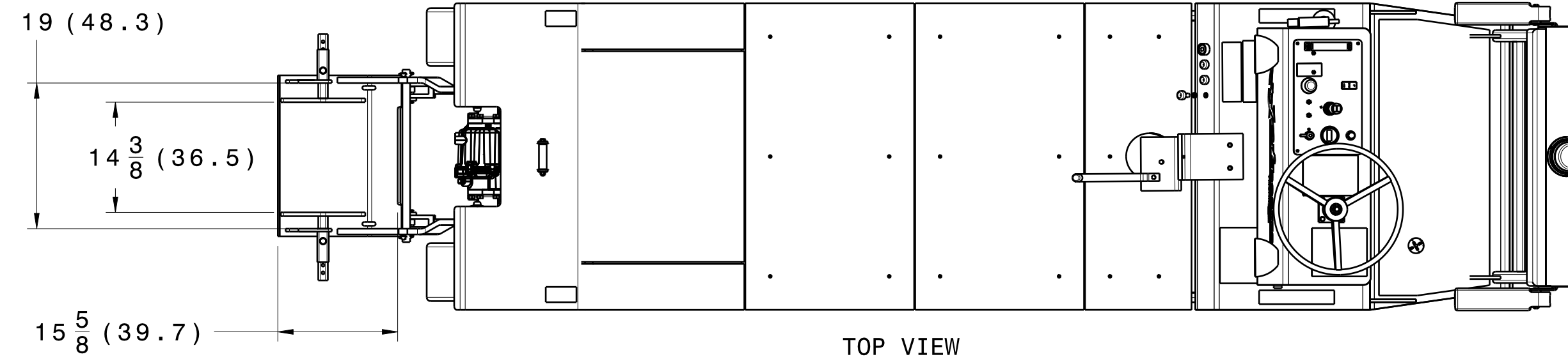
TOP VIEW
