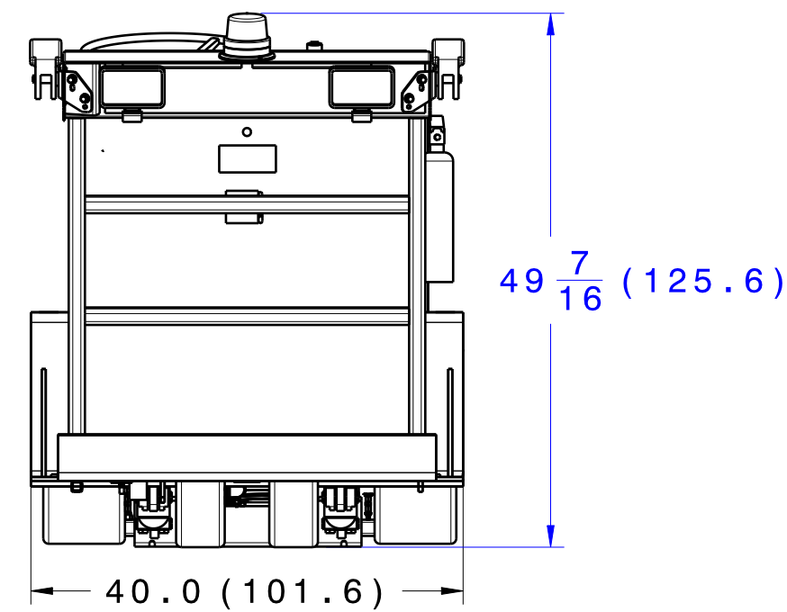
REAR VIEW
